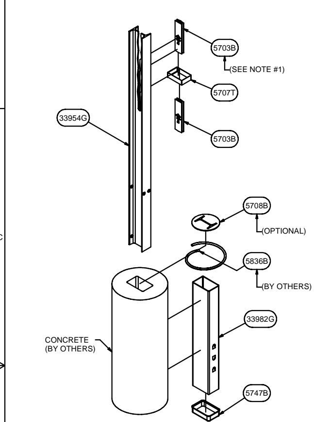
CASS-TL4 POST - IN CONCRETE (POST OPTION #3 - CAST IN PLACE)
