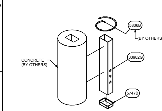
CONCRETE FOOTING ASSEMBLY (POST OPTION #3 - PRE-CAST OPTION)
