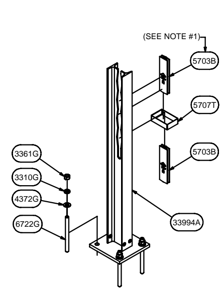
CASS-TL4 POST - BASE-PLATED (POST OPTION #5 - BASE-PLATED)
