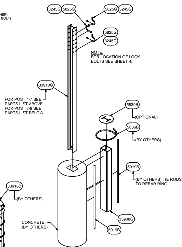
TERMINAL LINE POST - IN CONCRETE (CCT TERMINAL POST 4 - 7) (POST OPTION #1 SHOWN)
