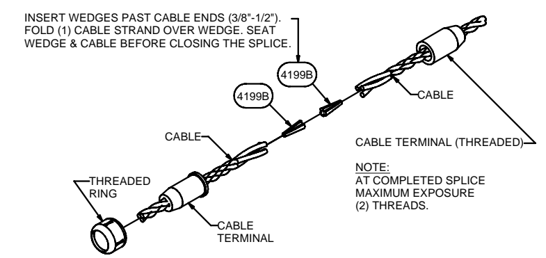
ASSEMBLY - TORPEDO CABLE SPLICE 4099G
