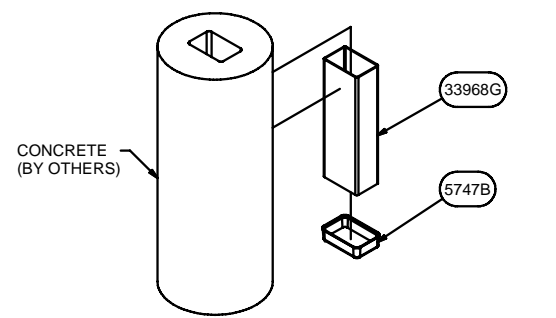
CONCRETE FOOTING ASSEMBLY (INSTALLED IN QUALIFYING MOW STRIP SEE CHART SHEET 1)
