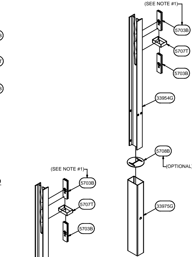
CASS-TL4 POST - IN DRIVEN SLEEVE (POST OPTION #6A - DRIVEN SLEEVE - NOTCH)
