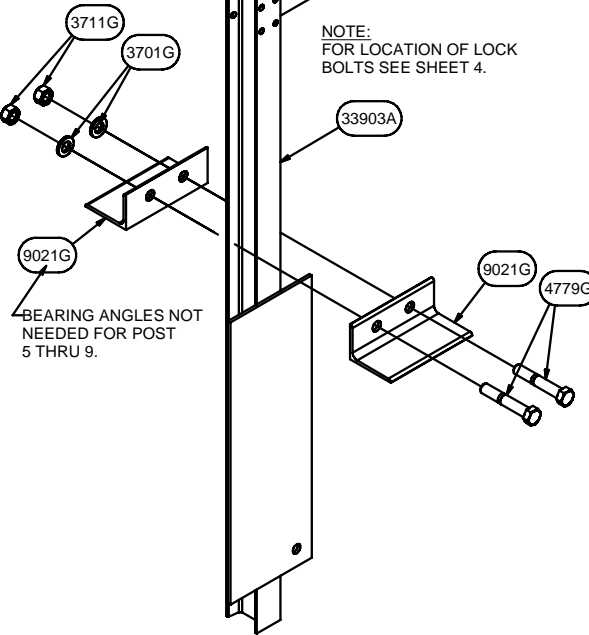
TERMINAL LINE POST - WITH SOIL PLATE (CCT TERMINAL POST - 4) (POST OPTION #2 SHOWN)
