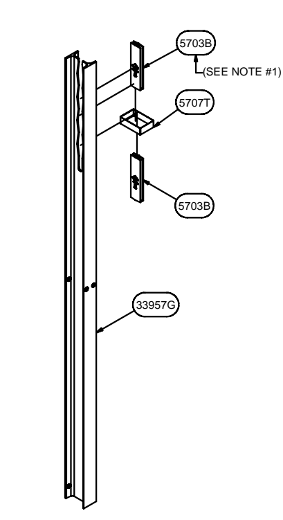
CASS-TL4 POST - DRIVEN (POST OPTION #4 - DRIVEN)
